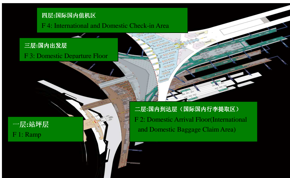
E 楼平面图 Ichnography of Building E
